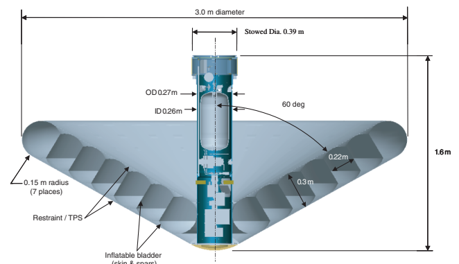
Fig. 4 Cross sectional view of IRVE, from [3].
